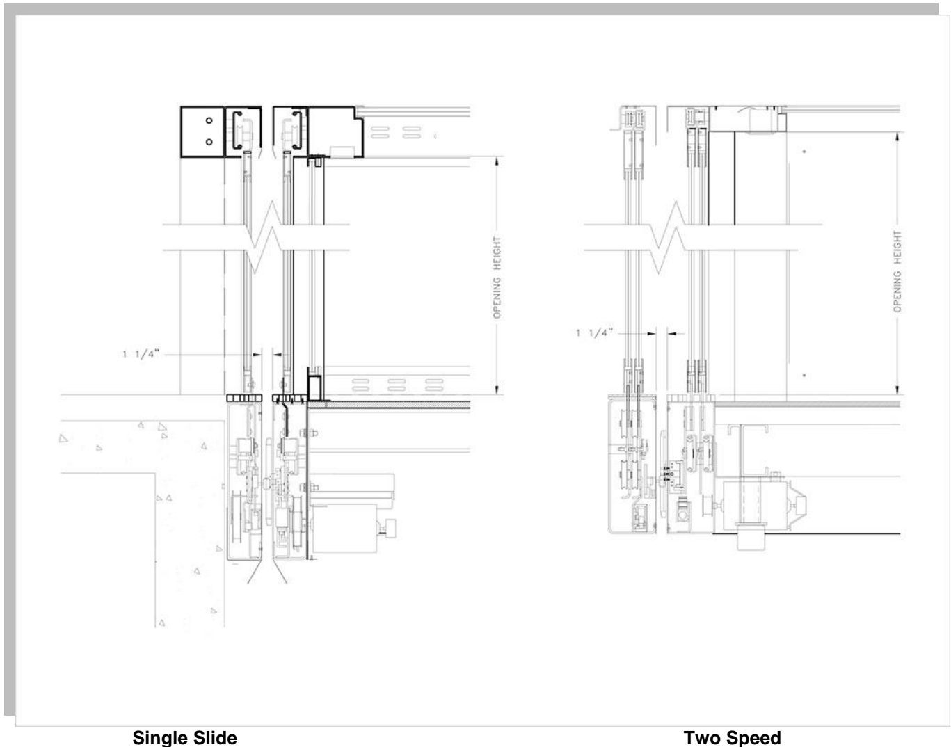
Section thru car and hall doors
